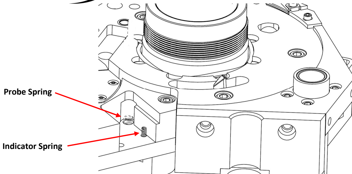
Figure 33 : Pace Probe Retractor and Indicator Springs in Spring Pockets as shown.
