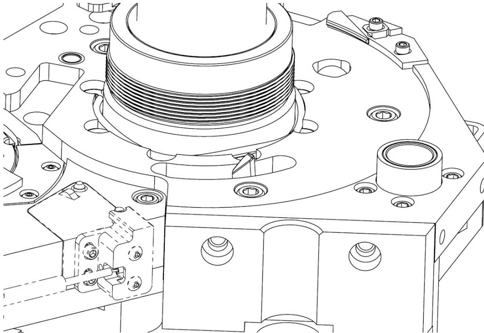
Figure 35: Primer Orientation Sensor Installed
