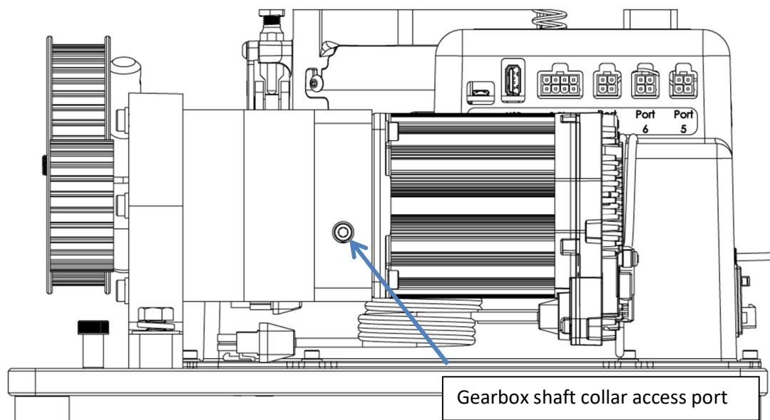
Figure 42: Gearbox Shaft connection
