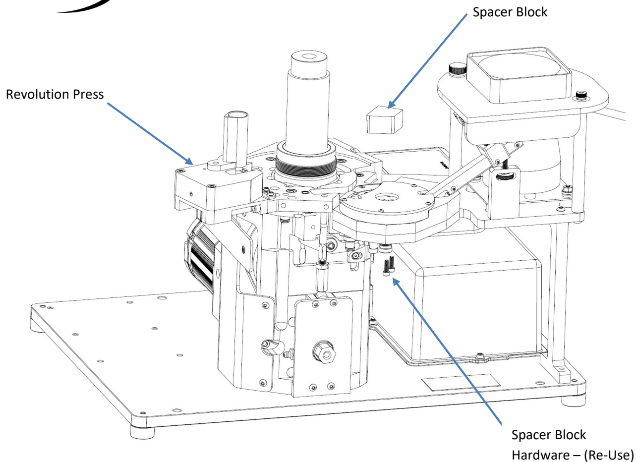
Figure 32 : Revolution Press Top End disassembled for Sensor Installation
