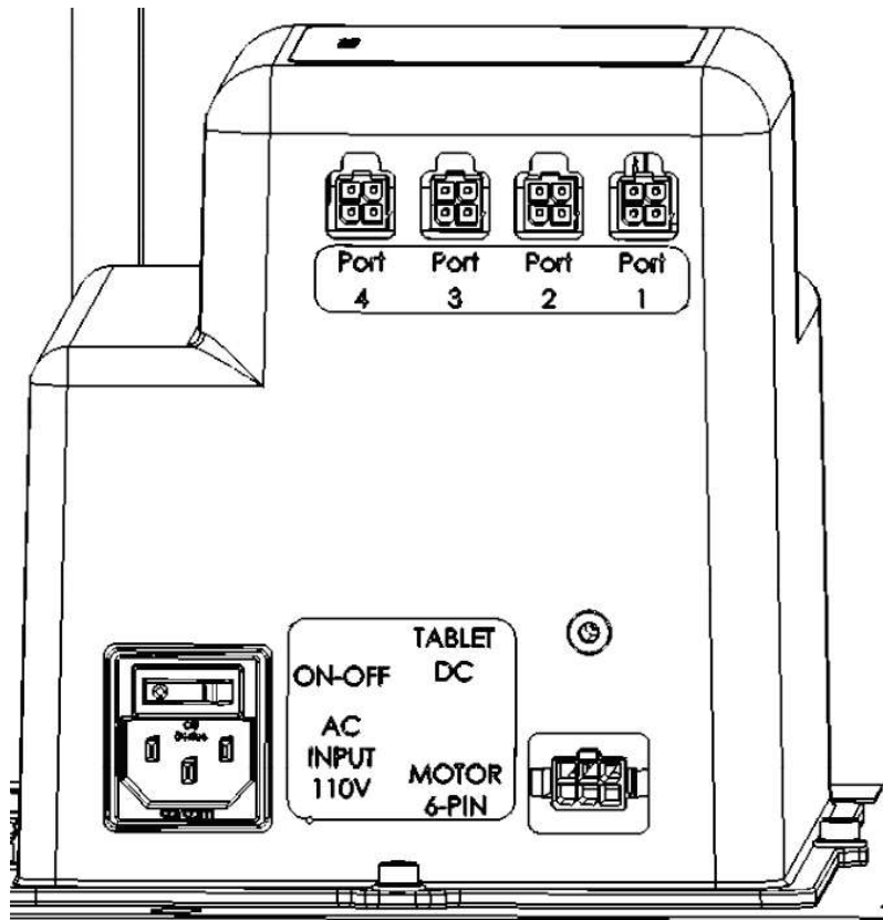
Figure 11: Side of Console Inputs
