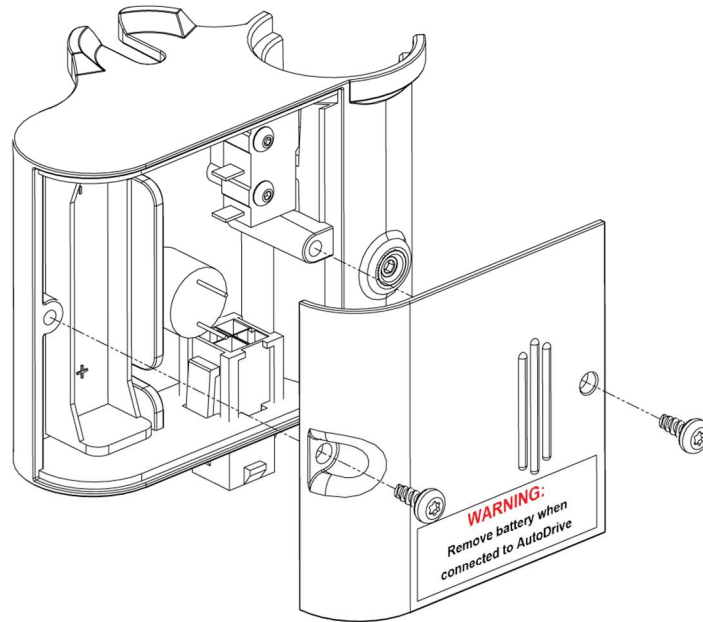
Figure 22: Removing Battery from PrimerSense
