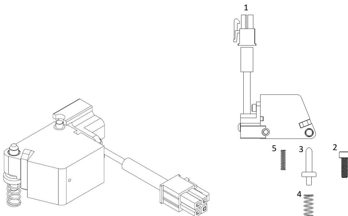
Figure 31: Primer Orientation Sensor
