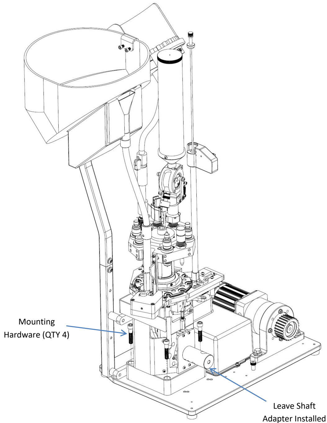
Figure 2 : Mounting Evolution to Baseplate
