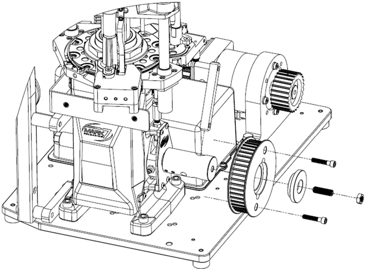
Figure 5: Mounting Large Sprocket on APEX 10
