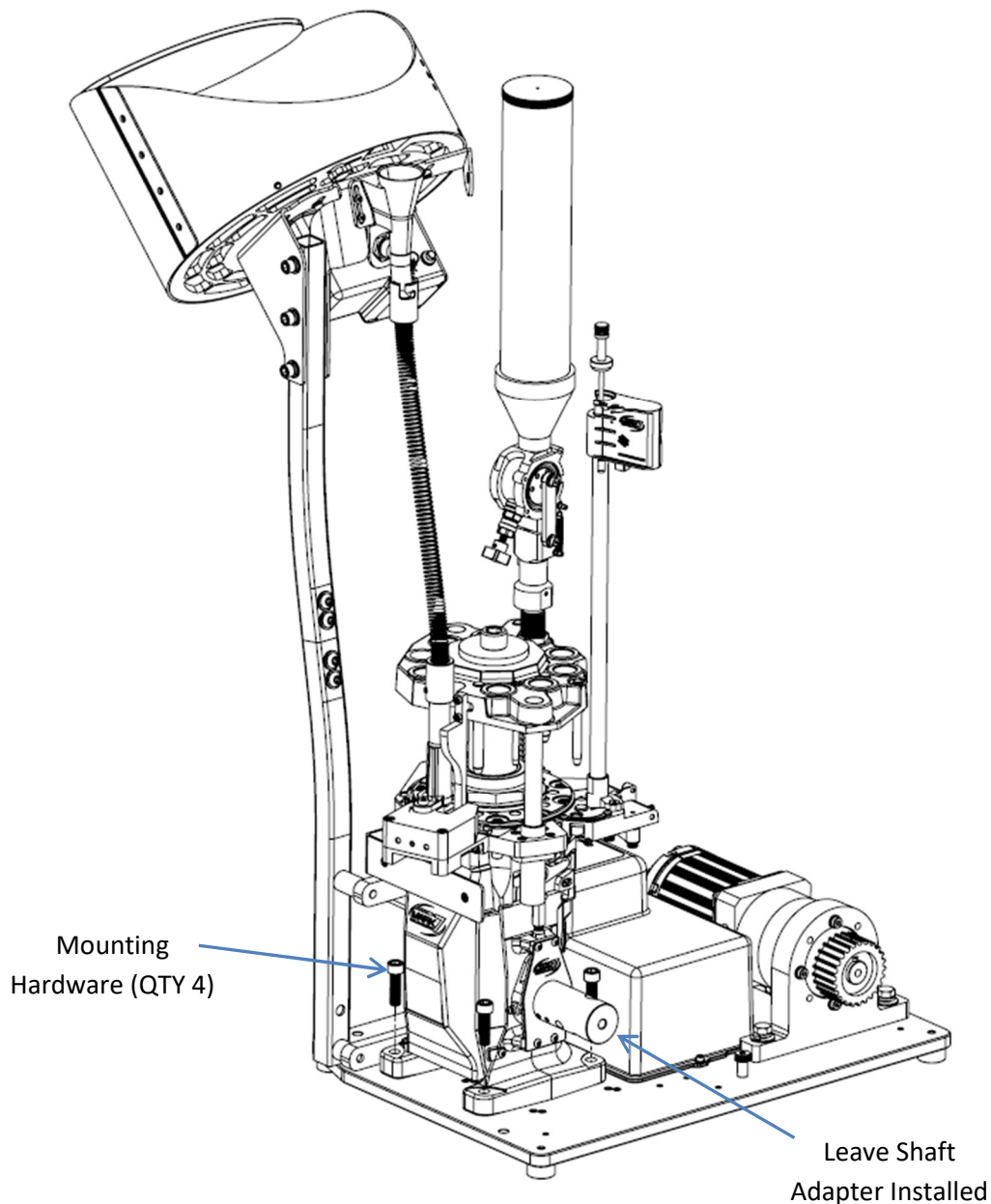
Figure 4 : Mounting APEX 10 to Baseplate
