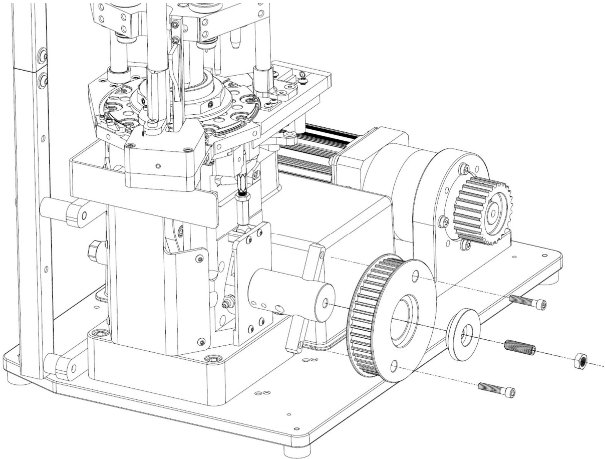
Figure 3: Mounting Large Sprocket on Evolution
