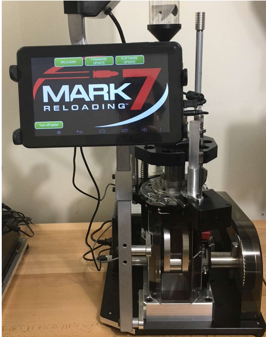
Figure 8: Tablet Installed in holder
