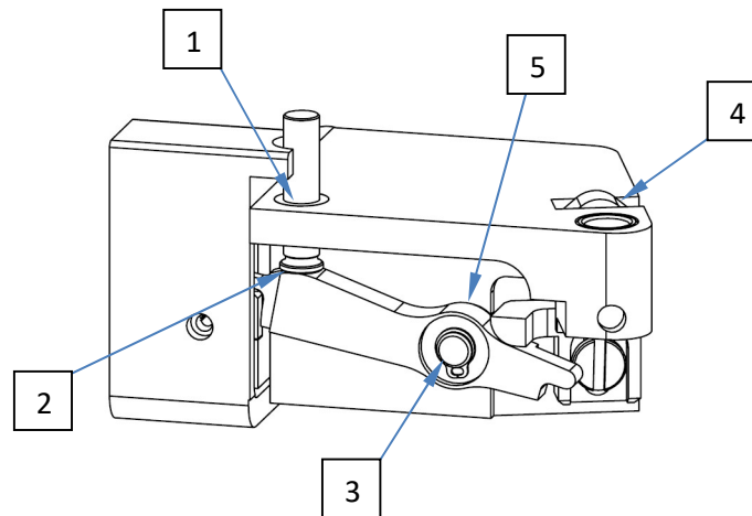
Figure 1: Primer Orientation Sensor lube points.
