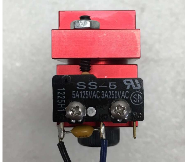
Figure 26: Micro switch Adjustment
