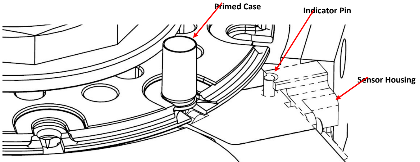
Figure 36 : Setting Optical Sensor Position
