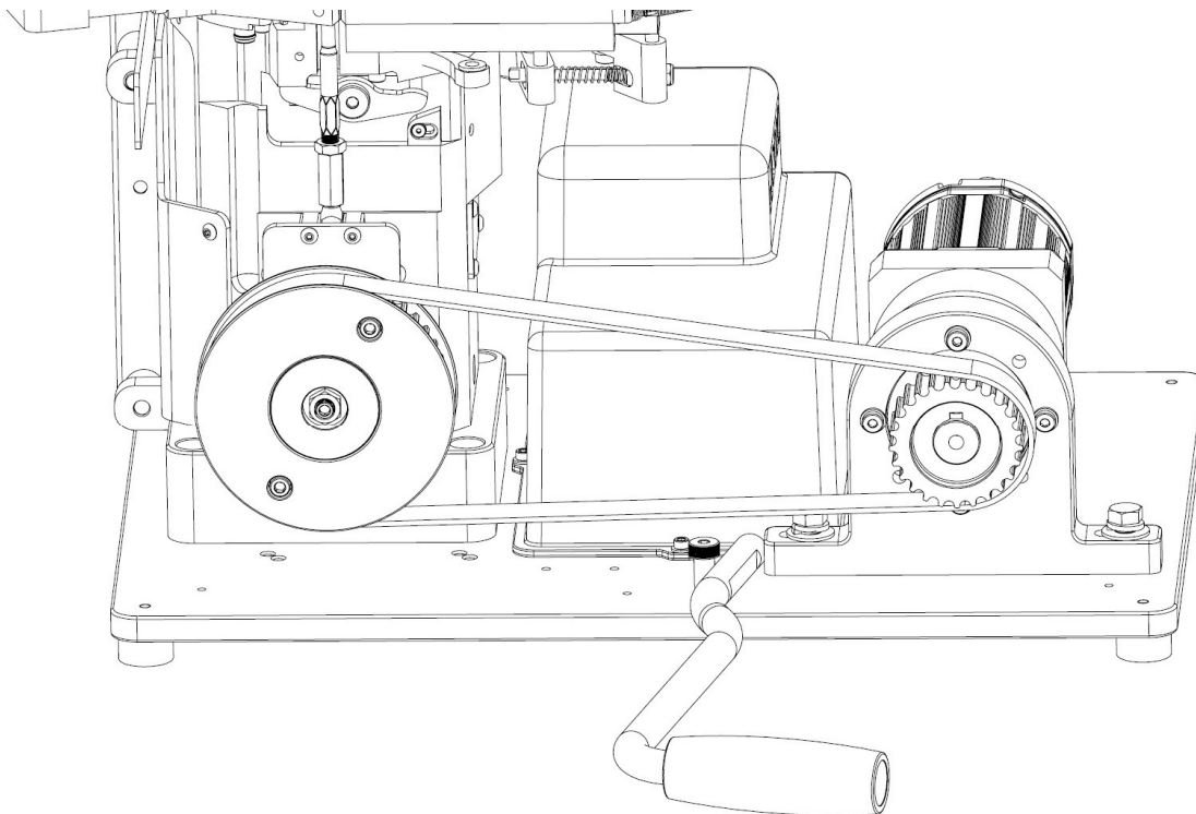
Figure 6: Installing the belt
