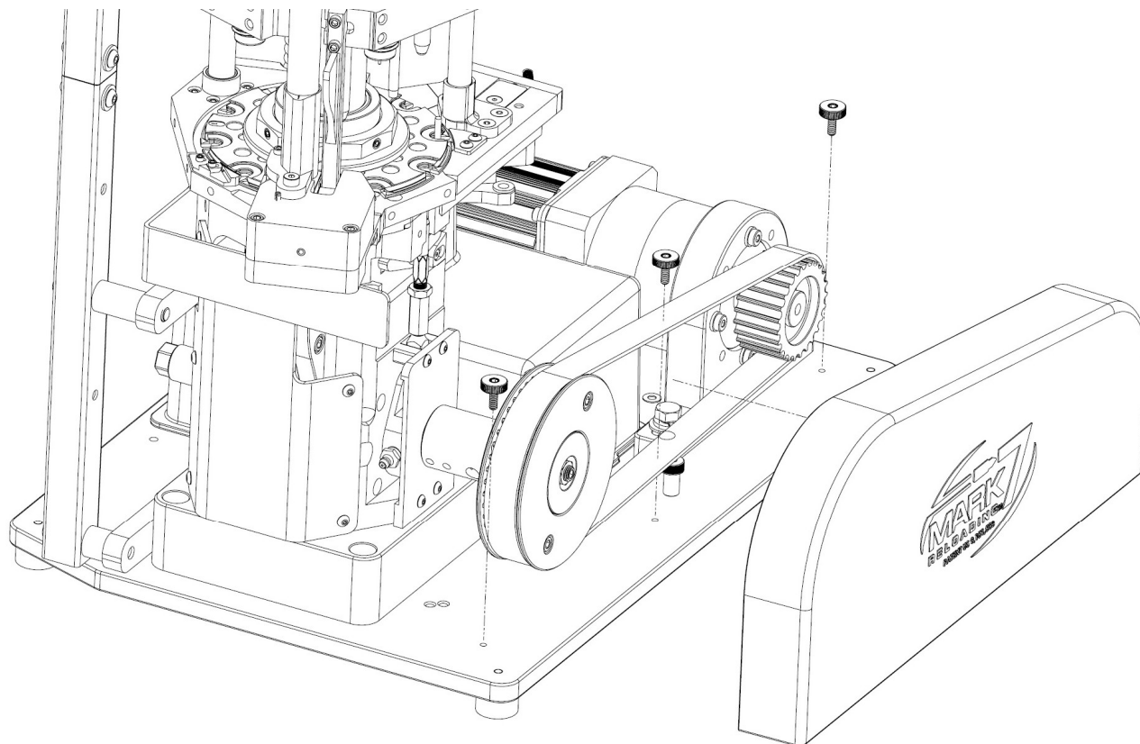
Figure 7: Installing Belt Guard
